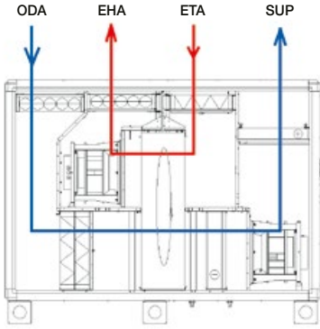
Arrangement diagram of components of Duovent® Compact RV TOP units without mixing (left position „L“)
