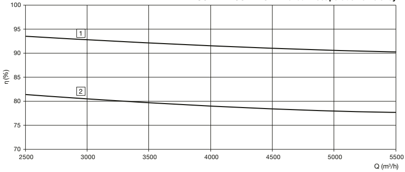
DUOVENT® COMPACT DV 5100 - recuperation efficiency
